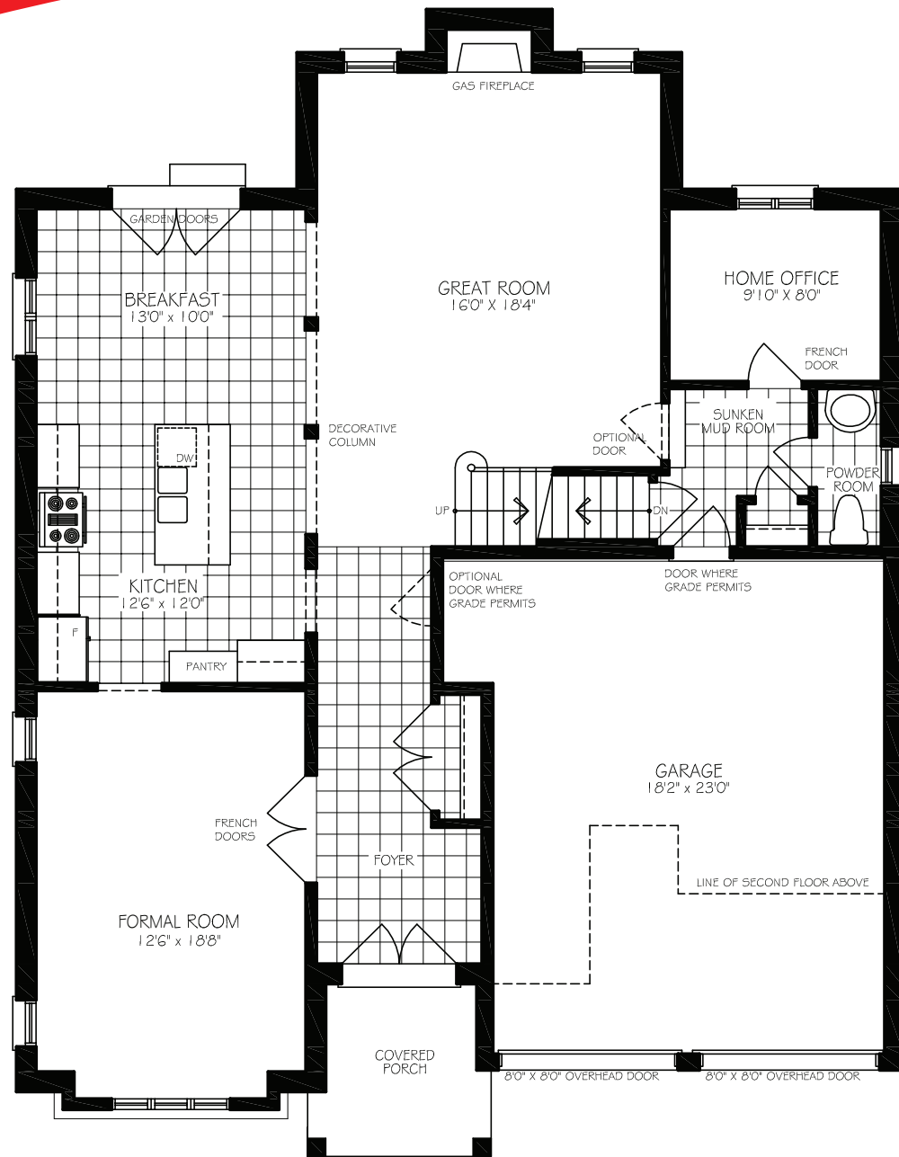
GROUND FLOOR PLAN - ELEVATION 'A'
