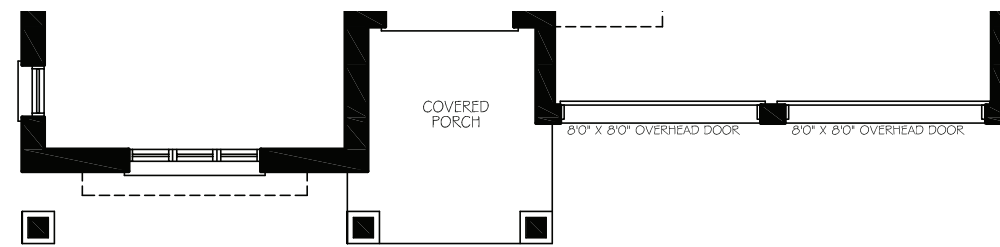
GROUND FLOOR PLAN - ELEVATION 'B'
