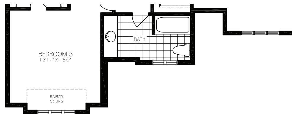
SECOND FLOOR PLAN - ELEVATION 'B'
