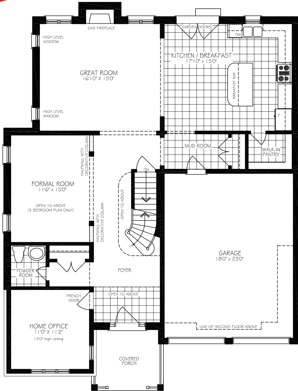
GROUND FLOOR PLAN - ELEVATION 'A'
