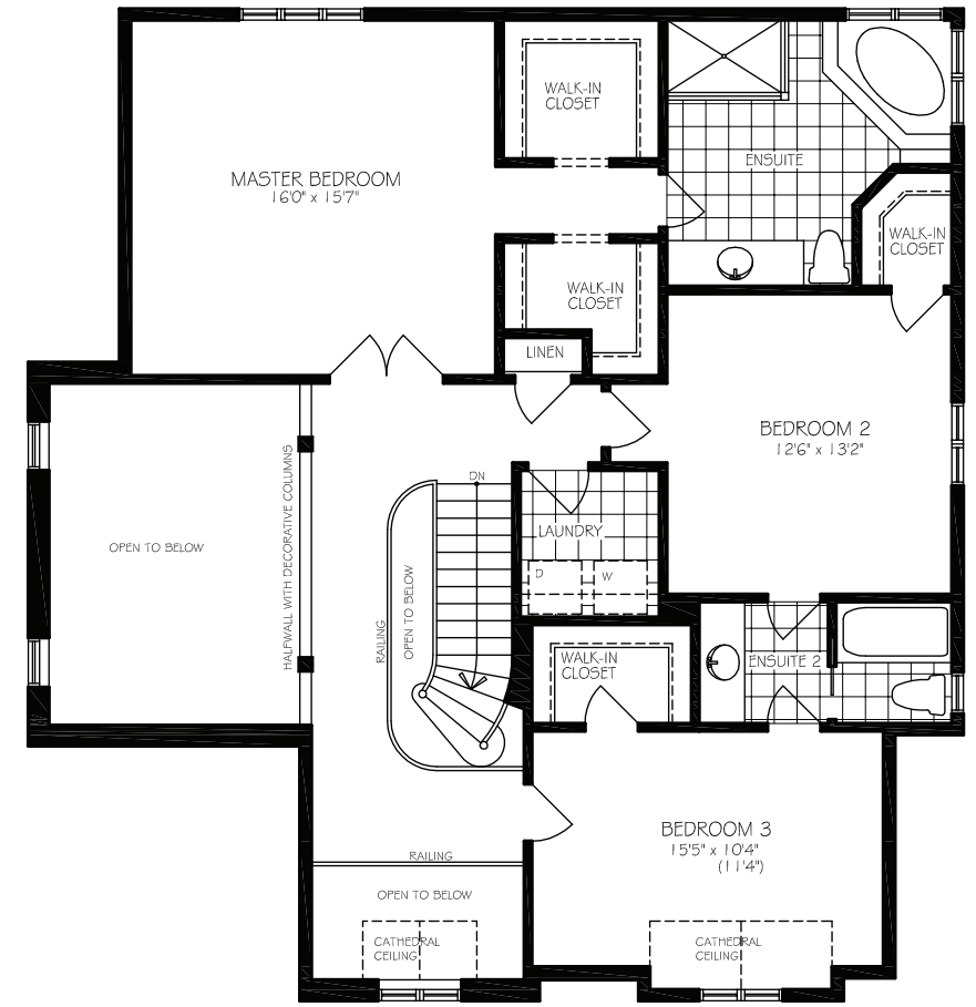
SECOND FLOOR PLAN - 3 BEDROOM - ELEVATION 'A'
