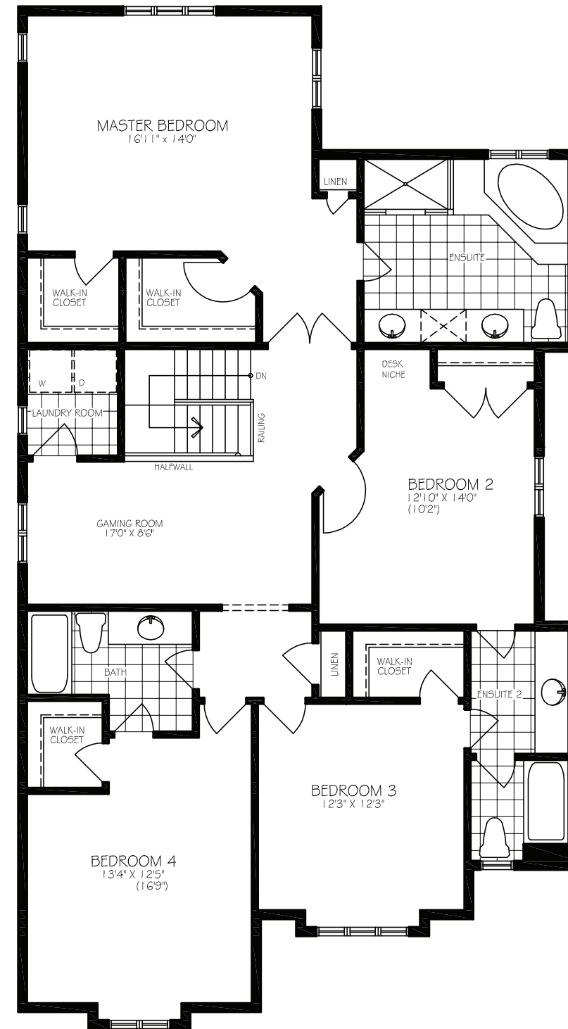
SECOND FLOOR PLAN - ELEVATION 'A'
