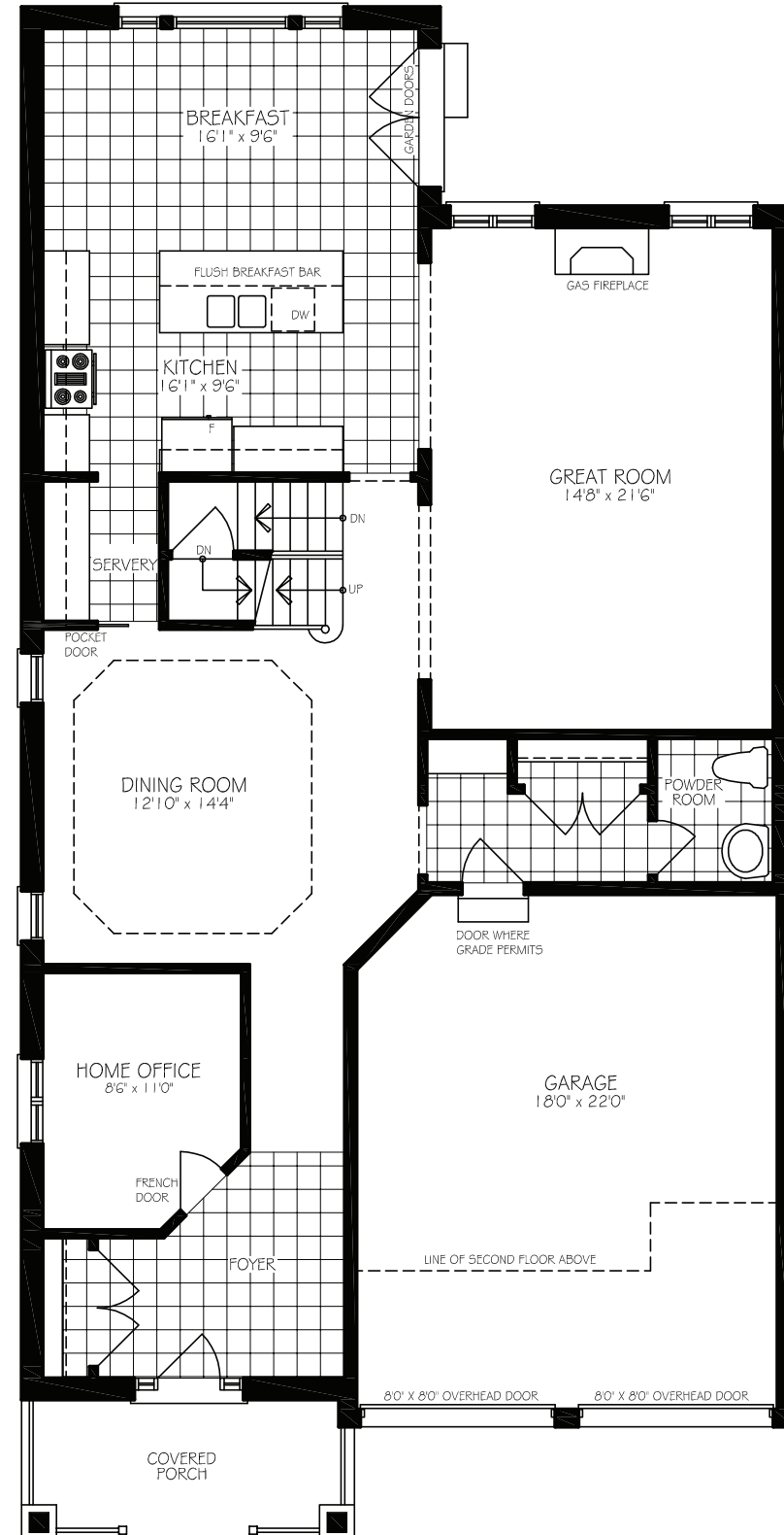
GROUND FLOOR PLAN - ELEVATION 'B'
