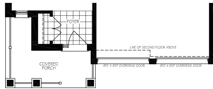
GROUND FLOOR PLAN - ELEVATION 'B'
