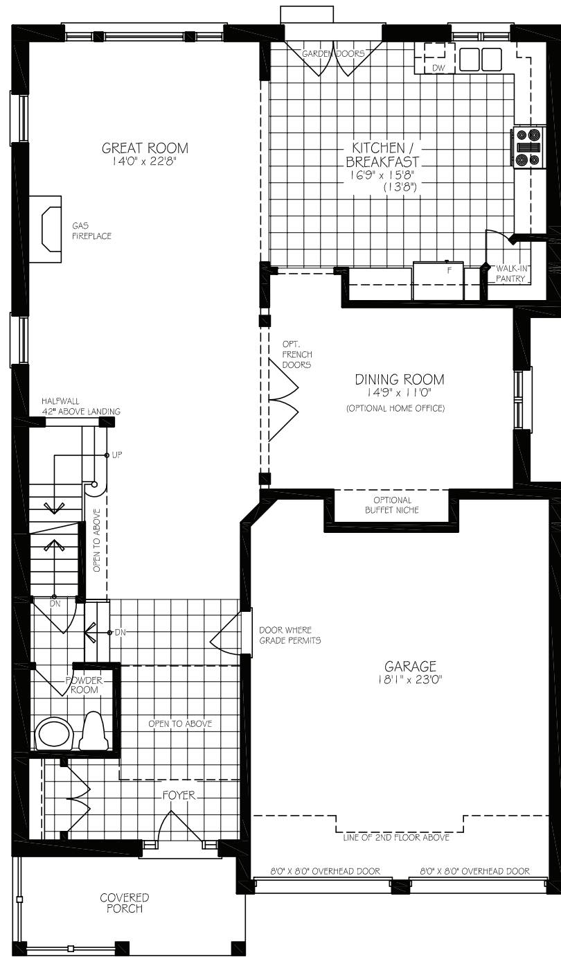
GROUND FLOOR PLAN - ELEVATION 'A'
