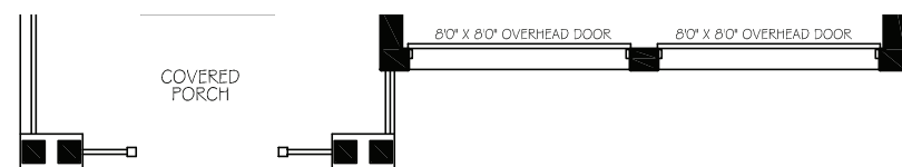
GROUND FLOOR PLAN - ELEVATION 'B'
