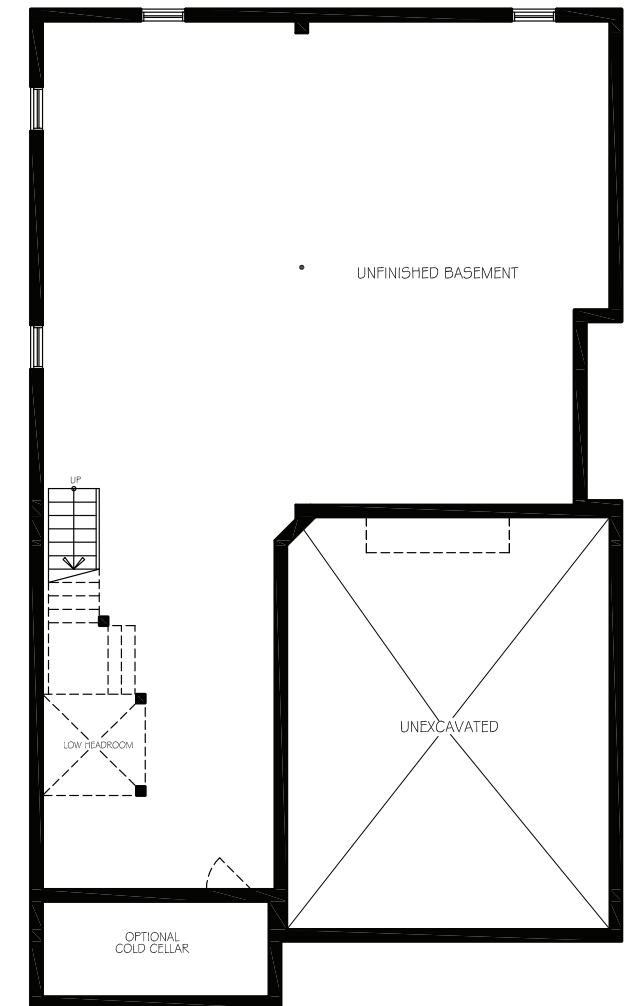
BASEMENT PLAN - ELEVATION 'A'
