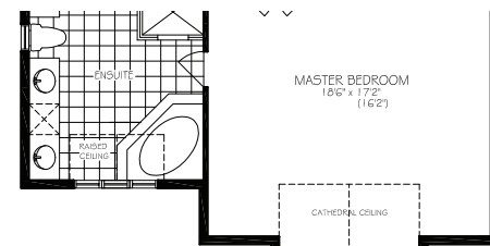
SECOND FLOOR PLAN - ELEVATION 'B' - 4 BEDROOM PLAN
