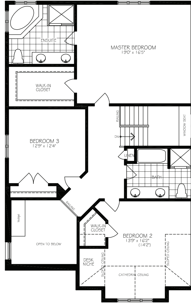
SECOND FLOOR PLAN - ELEVATION 'A' - 3 BEDROOM PLAN
