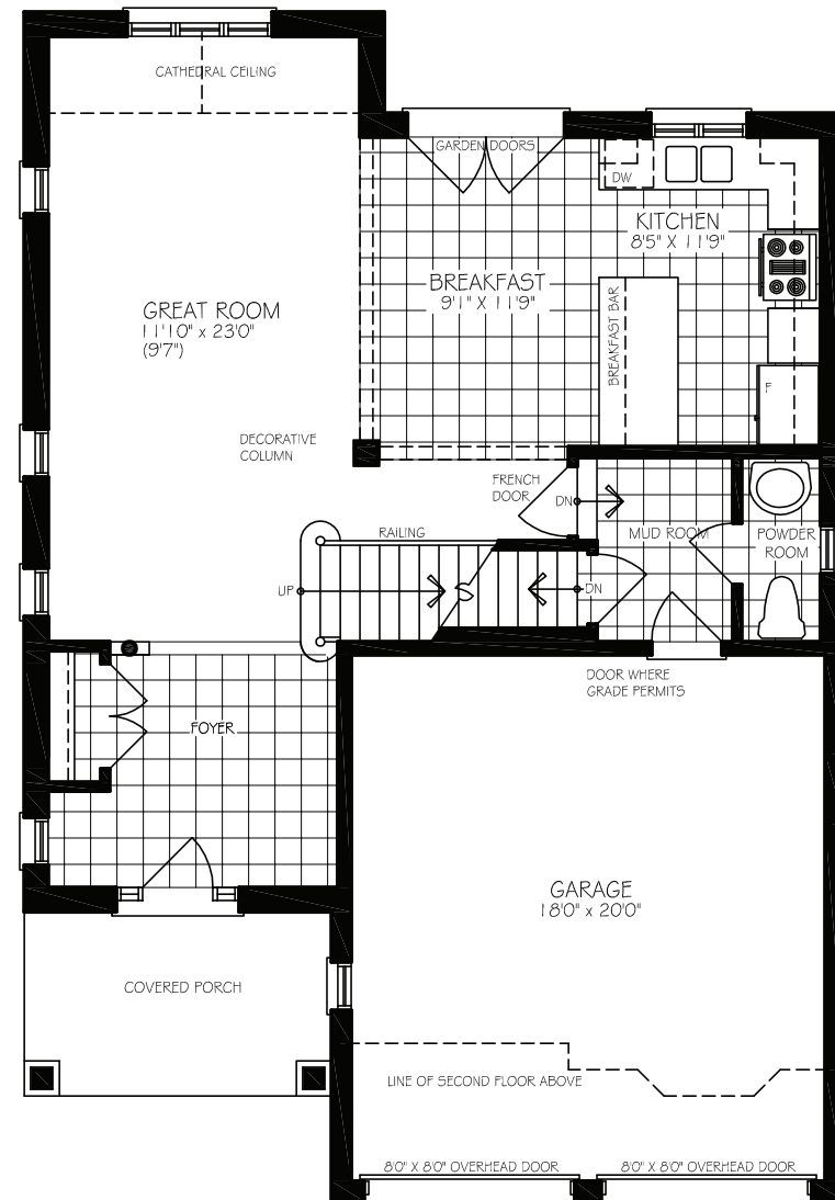
GROUND FLOOR PLAN - ELEVATION 'B'
