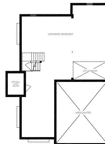
BASEMENT PLAN - ELEVATION 'B'
