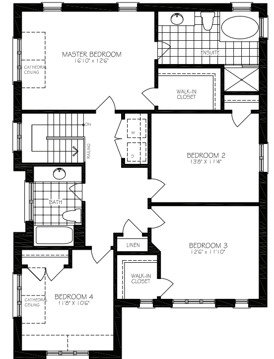
ALTERNATE SECOND FLOOR PLAN - ELEVATION 'A'
