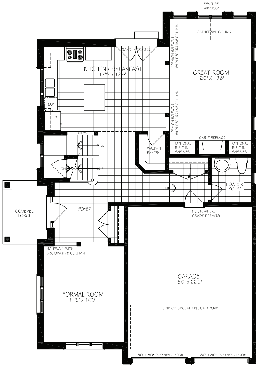
GROUND FLOOR PLAN - ELEVATION 'A'
